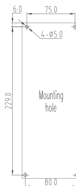
M2(5.5KW)' s dimensions, the unit is mm
